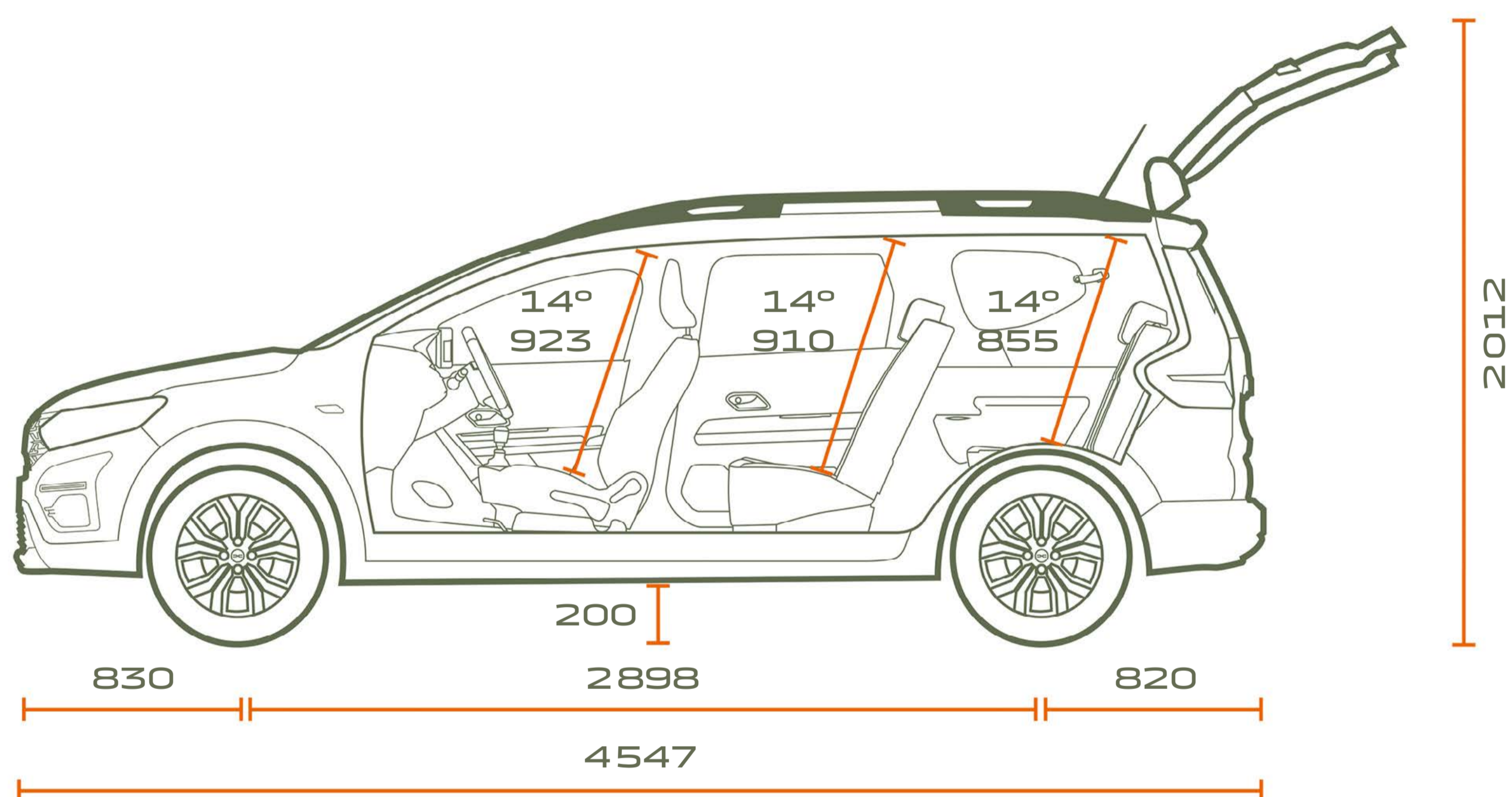
SIDE VIEW
