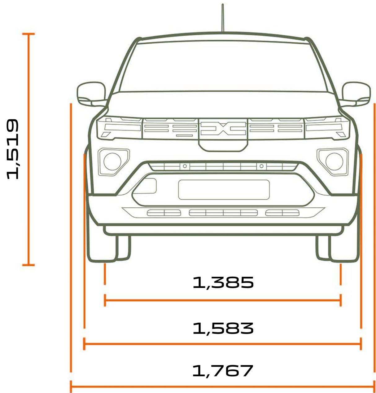
FRONT VIEW
