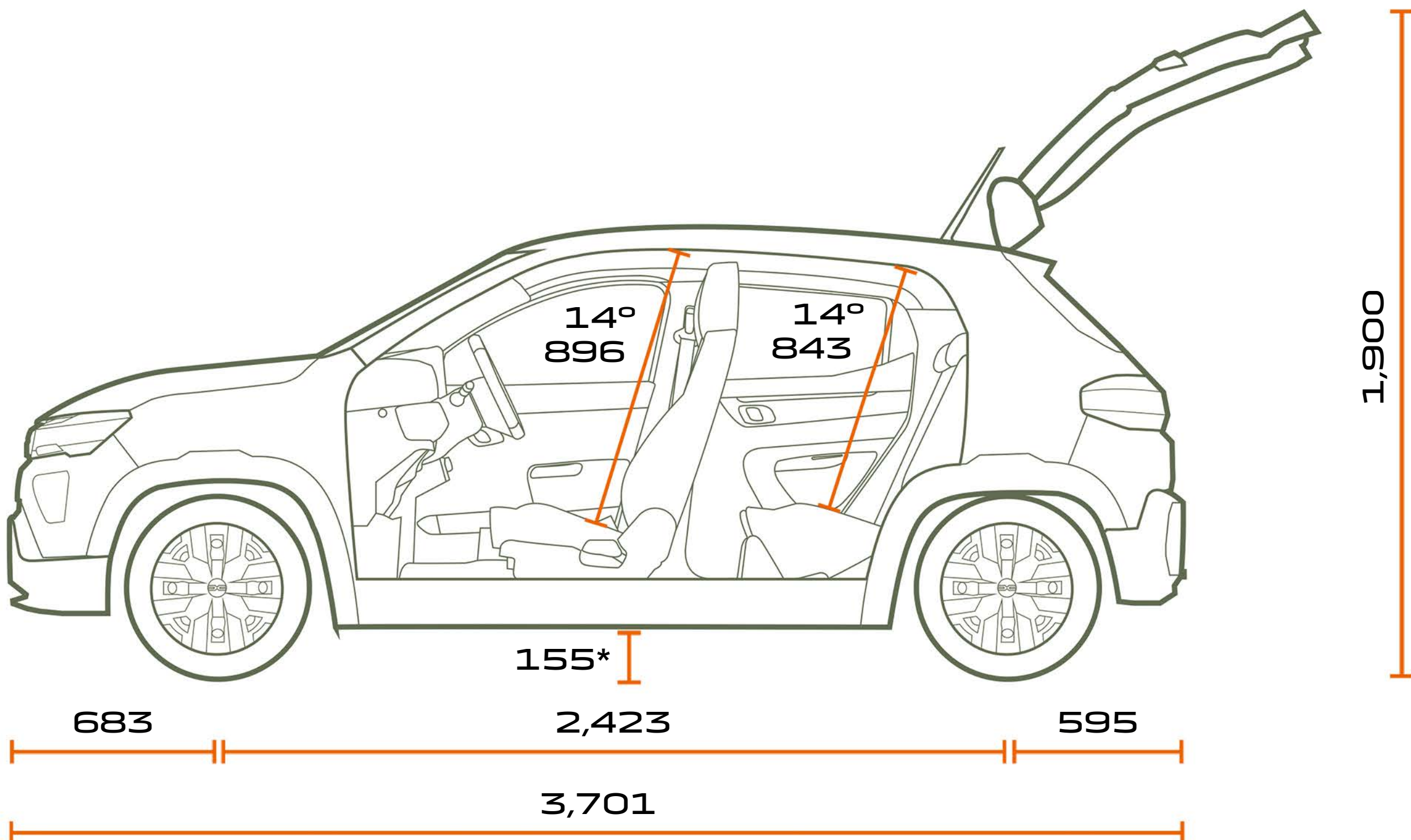
SIDE-FACE VIEW
