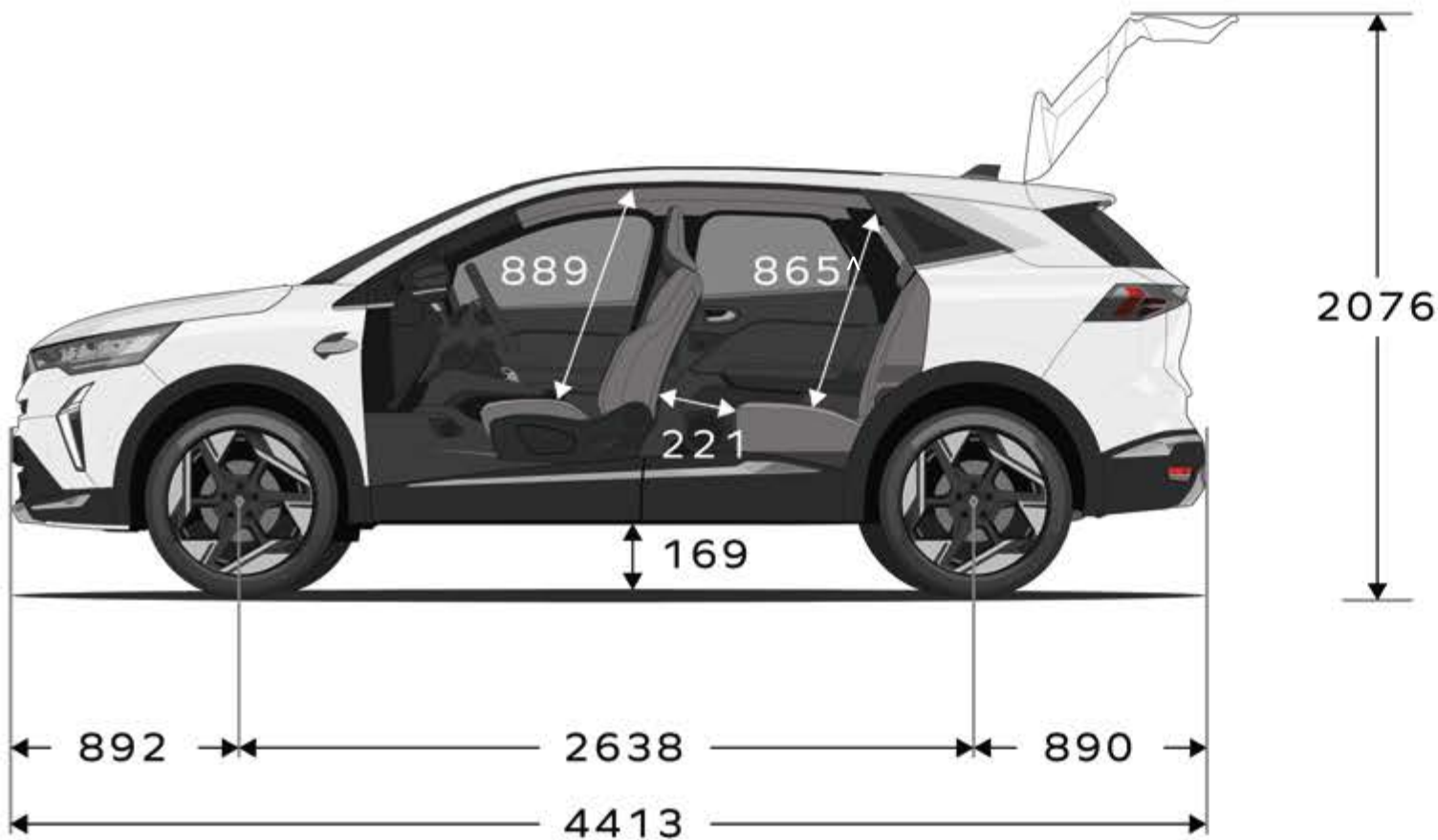
^rear 2nd row headroom with Solarbay
