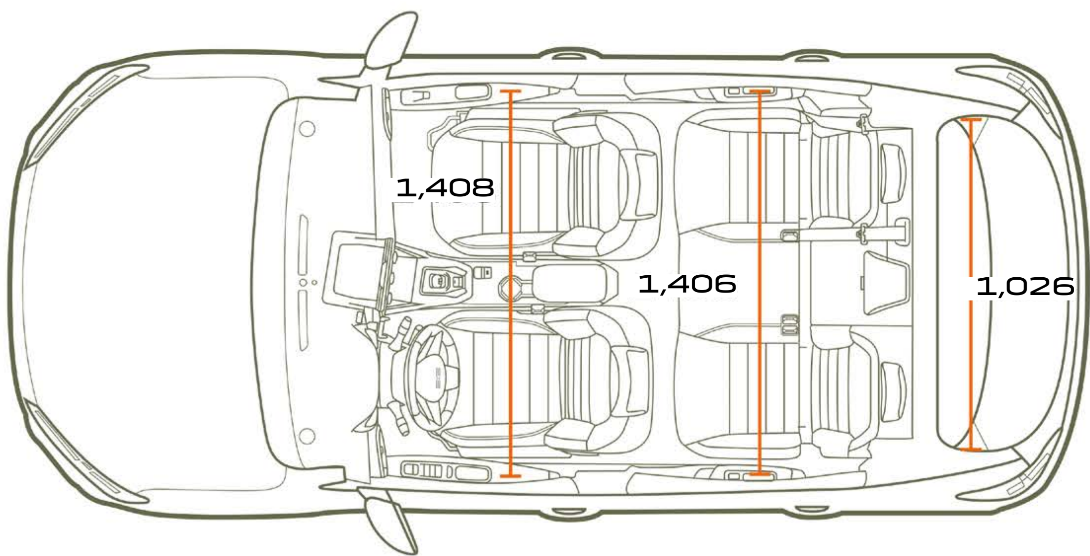
TOP VIEW
