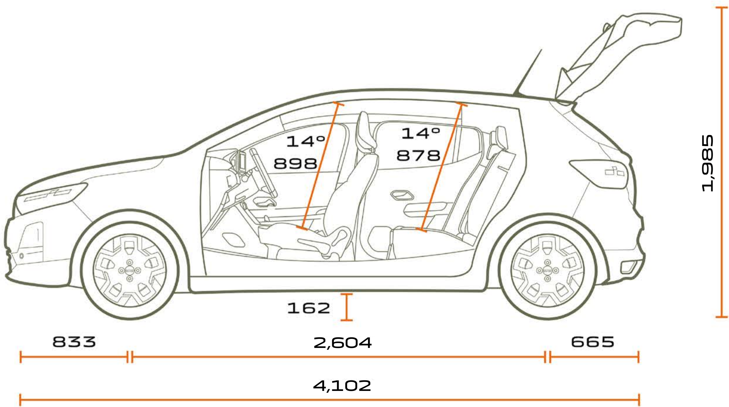
SIDE VIEW
