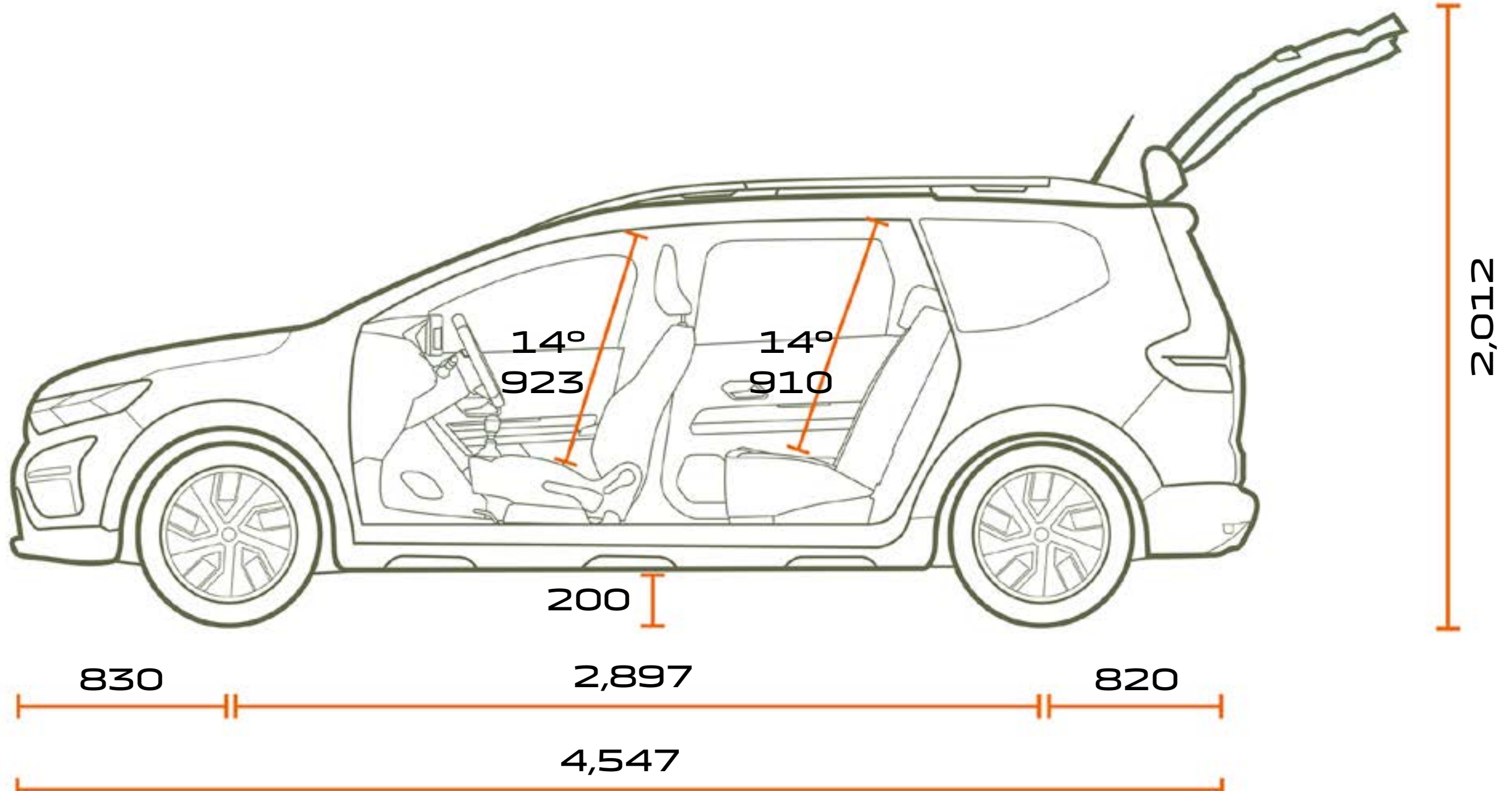
5-SEATER SIDE VIEW
