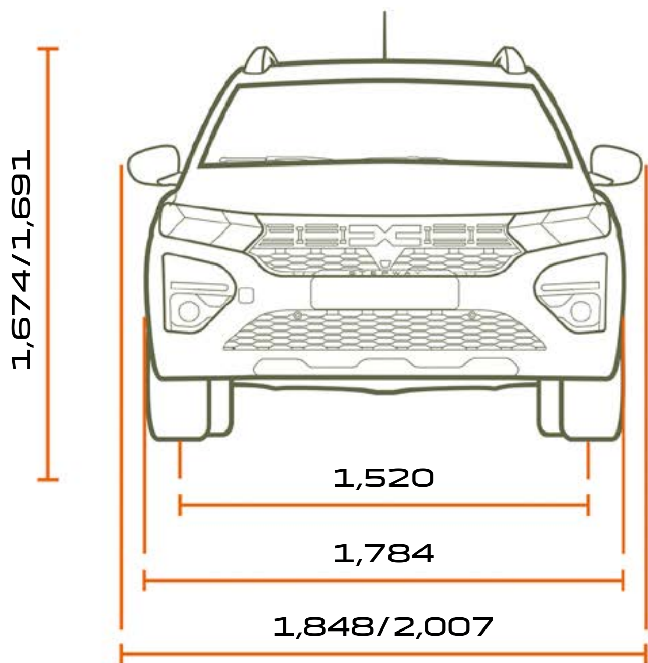
FRONT VIEW 5 AND 7 SEATERS
